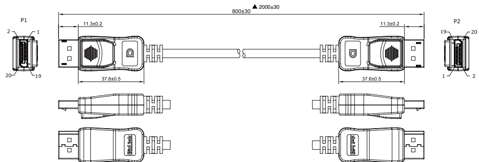
DP40 Enhanced Full-Size DP 2 Meter Twist-Pair/Coaxial
