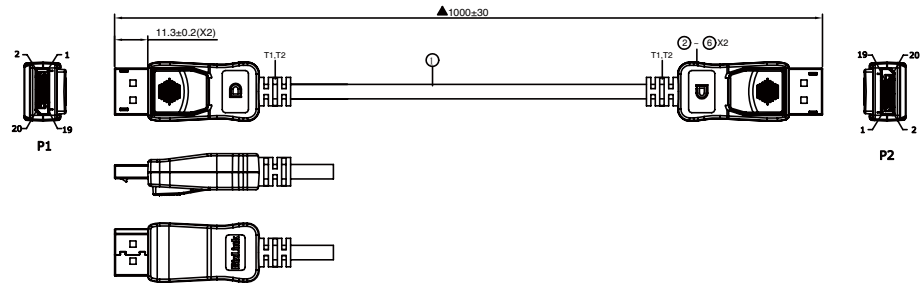
DP80 Enhanced Full-Size DP 1 Meter Twist-Pair/Coaxial
