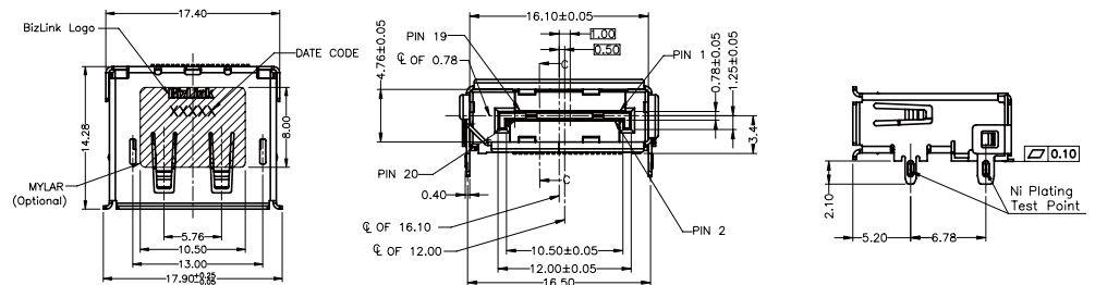
DP80 Enhanced Full-Size DP Receptacle Connectors
